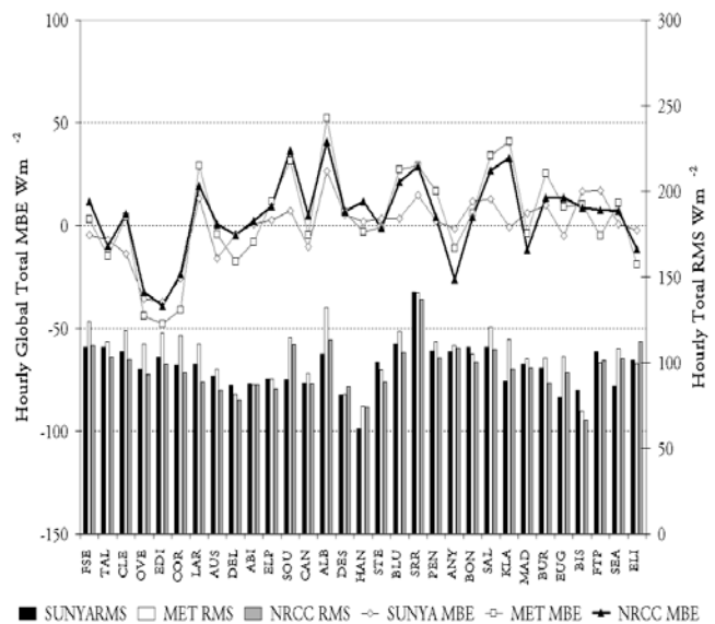
Fig. 2. MBE (lines, left scale) and RMSE (bars, right scale) for modeled hourly total GHI by site and by model. From (11).
