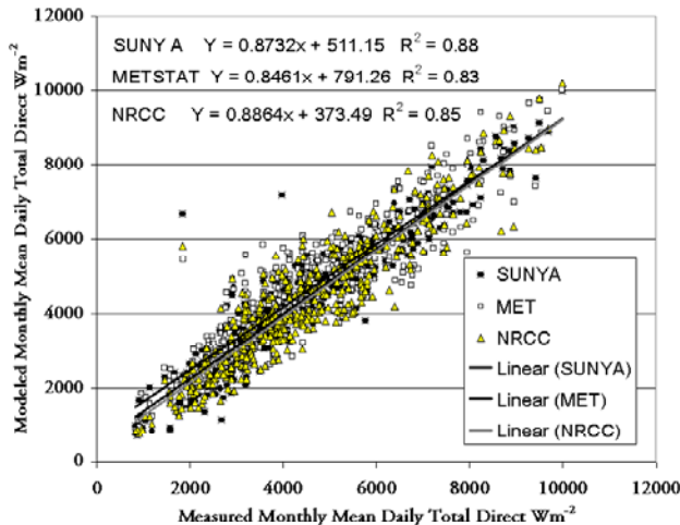
Fig. 3. Modeled versus measured DNI monthly mean daily totals, regression fit, and correlation coefficients by model.
